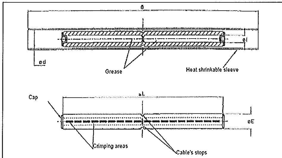
Fig 1: sleeve joint
